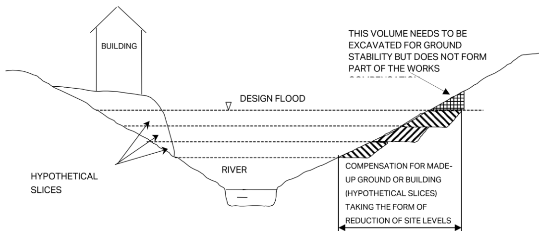
Figure 5-1 Example of Floodplain Compensation Storage (Environment Agency 2009)
